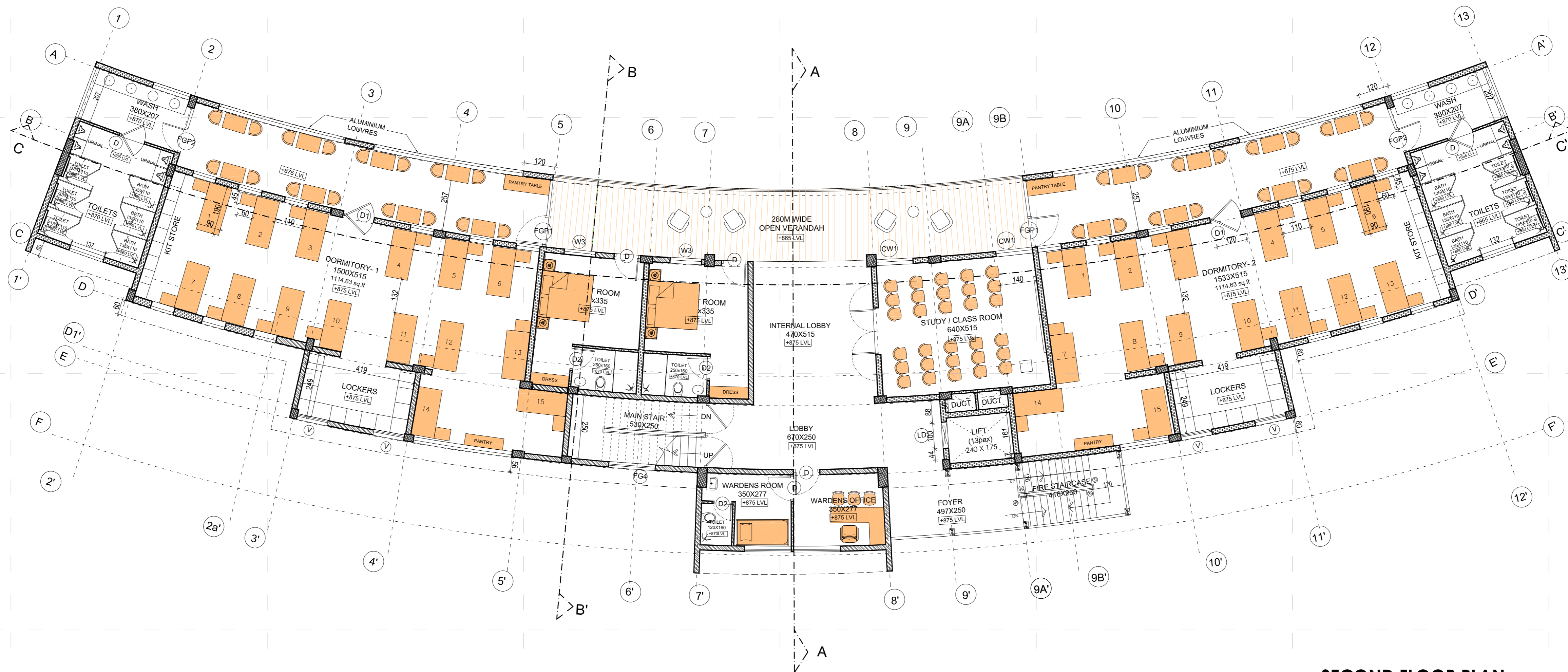
SECOND FLOOR PLAN SCALE 1:100
